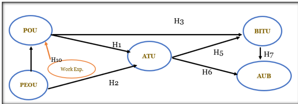
Figure 2: Result Model
